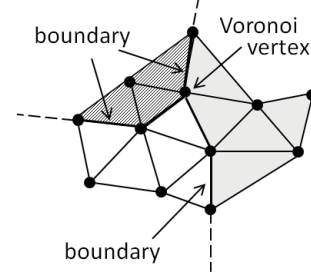
Figure 5. Voronoi vertex
