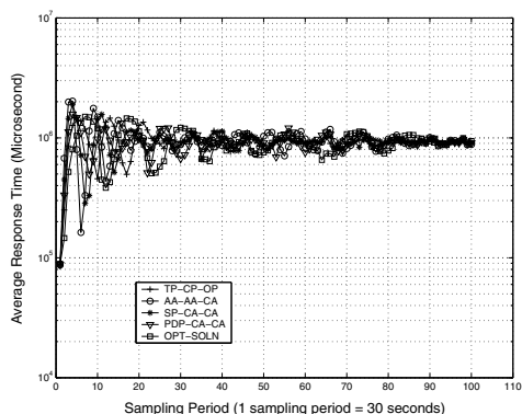
Figure 7. Integrated Algorithms: Time
