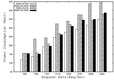
Figure 6. Effects of Activation Thresholds and Workload Distribution: Power
