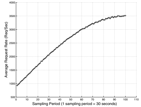
Figure 2. Average Request Rate
