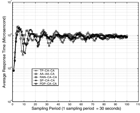
Figure 3. Effects of Ordered Server List: Time
