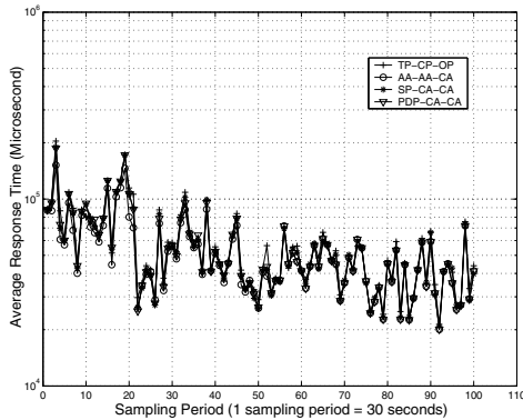
Figure 9. Effects of Feedback Control: Time
