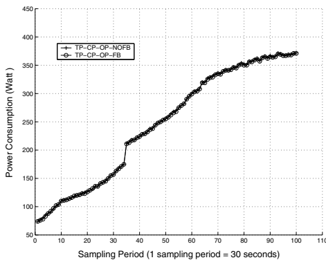
Figure 10. Effects of Feedback Control: Power
