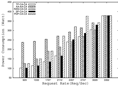
Figure 4. Effects of Ordered Server List: Power
