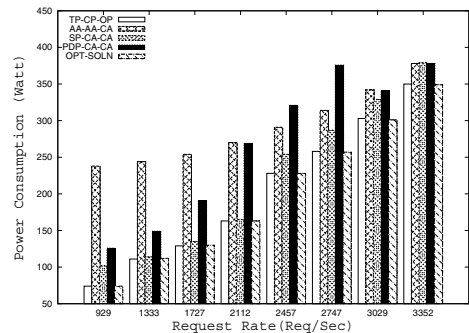
Figure 8. Integrated Algorithms: Power
